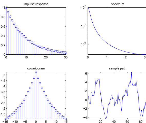
Figure 2.10.2: Impulse response, spectrum, covariogram, and sample path of process (1 - .9L)y_t = w_t .
