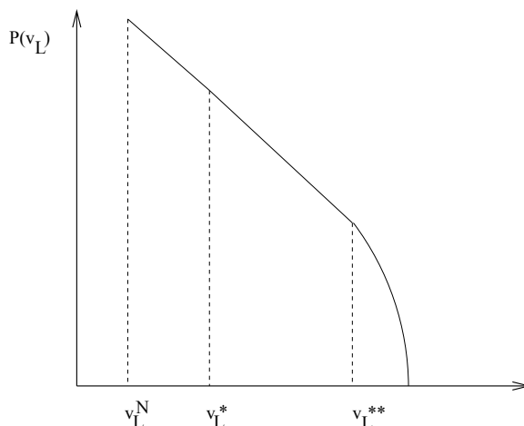
Figure 25.3.1: The constrained Pareto frontier v_S = P(v_L) in the Bond-Park model.
