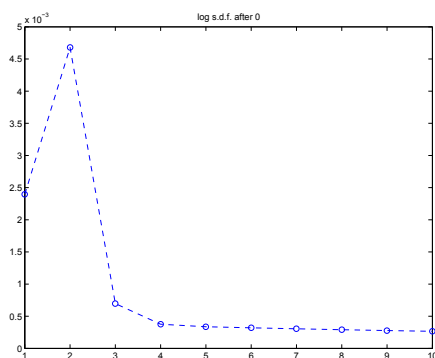
Figure 14.B.4: Impulse response of log stochastic discount factor from lag 1 on.
