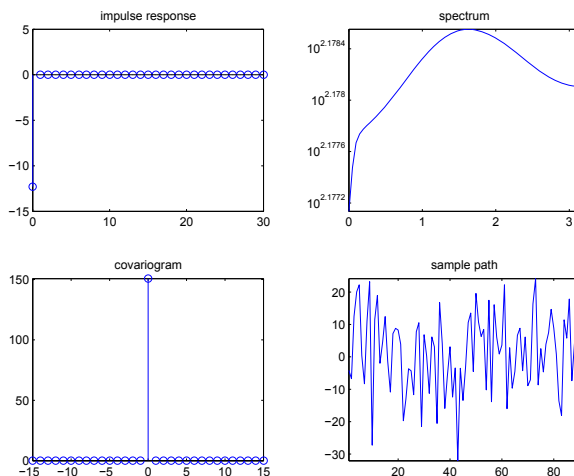
Figure 14.B.5: bigshow2 for Backus and Zin's log stochastic discount factor.
