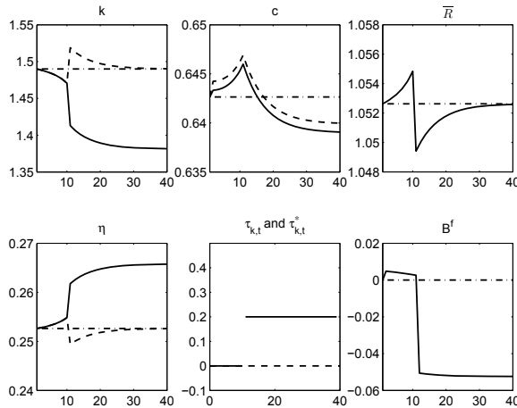
Figure 11.13.3: Response to once-and-for-all increase in \tau_k at t = 10 foreseen at time t = 1 . From left to right, top to bottom: k , c , \bar{R} , \eta , \tau_k and \tau_k^* , and B^f . Domestic country (solid line), foreign country (dotted line) and steady-state values (dot-line).
