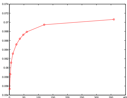
Figure 14.B.1: Mean term structure of interest rates with Backus-Zin stochastic discount factor (months on horizontal axis).
