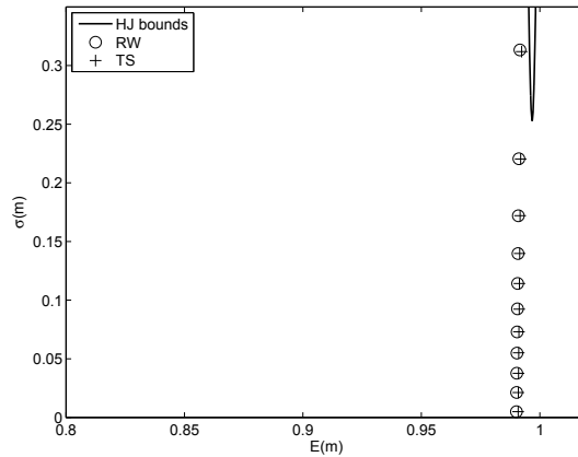
Figure 14.8.1: Reciprocal of risk free rate, market price of risk pairs for the random walk ( \oplus ) model for values of detection error probabilities of 50, 45, 40, 35, 30, 25, 20, 15, 10, 5 and 1 percent.
