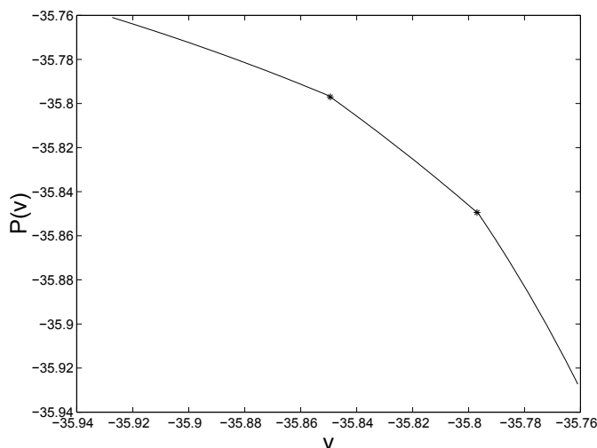
Figure 21.11.4: Pareto frontier P(v) for the three-state symmetric example. Kinks occur at coordinates (v, P(v)) = (w^-, w^+) and (v, P(v)) = (w^+, w^-) .
